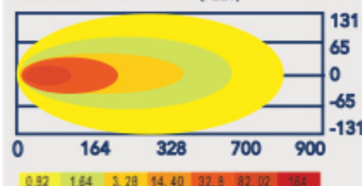
BEAM PATTERN (FEET)
