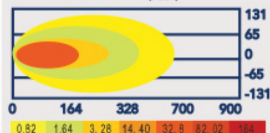
BEAM PATTERN (FEET)
