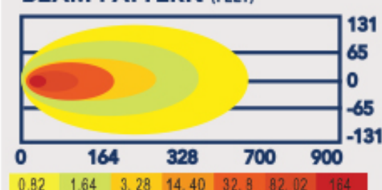
BEAM PATTERN (FEET)
